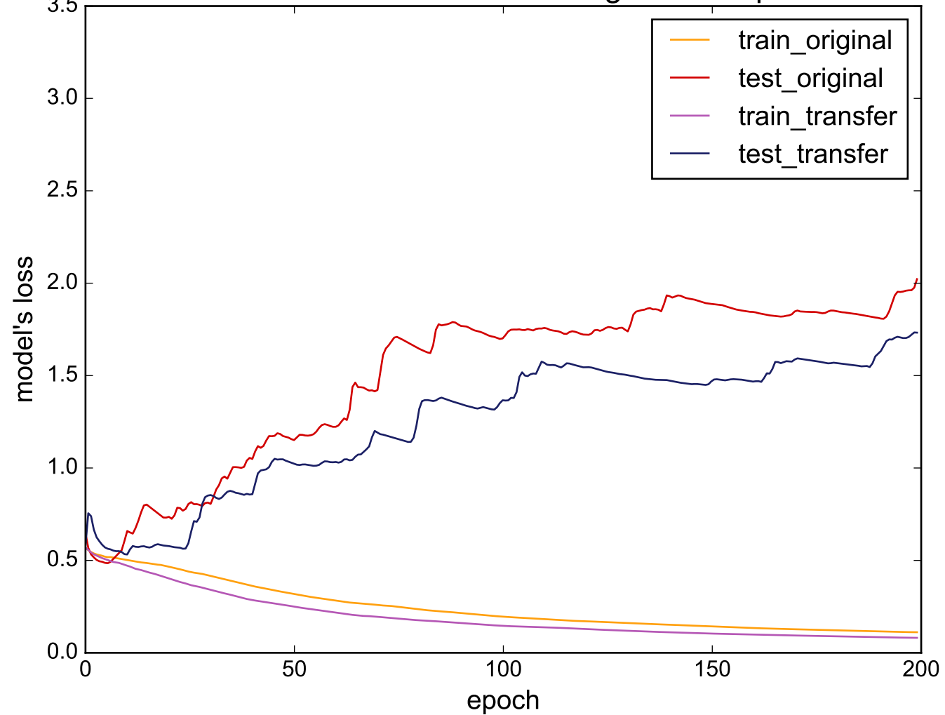
Source: DistalPhalanxTW - Target: Earthquakes
