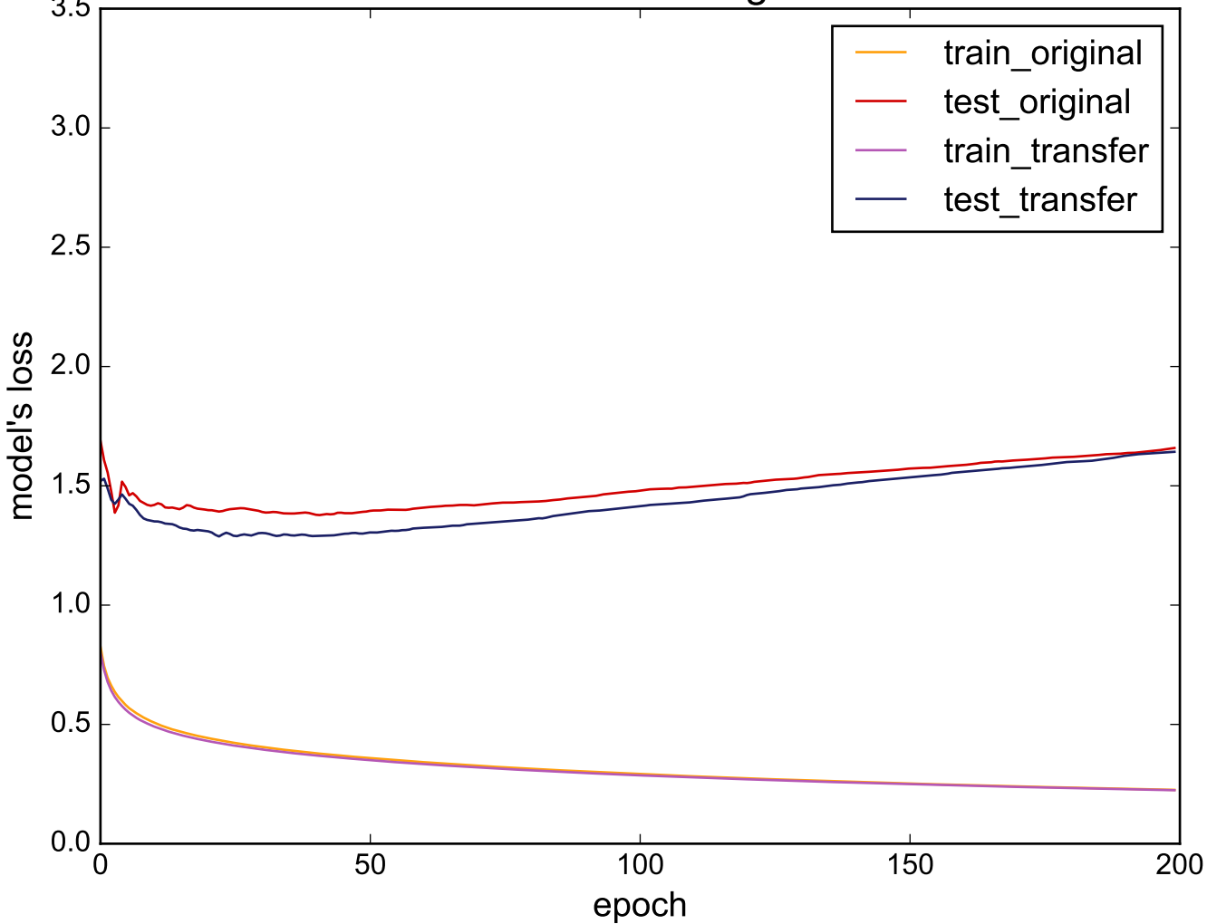
Source: DistalPhalanxTW - Target: ElectricDevices
