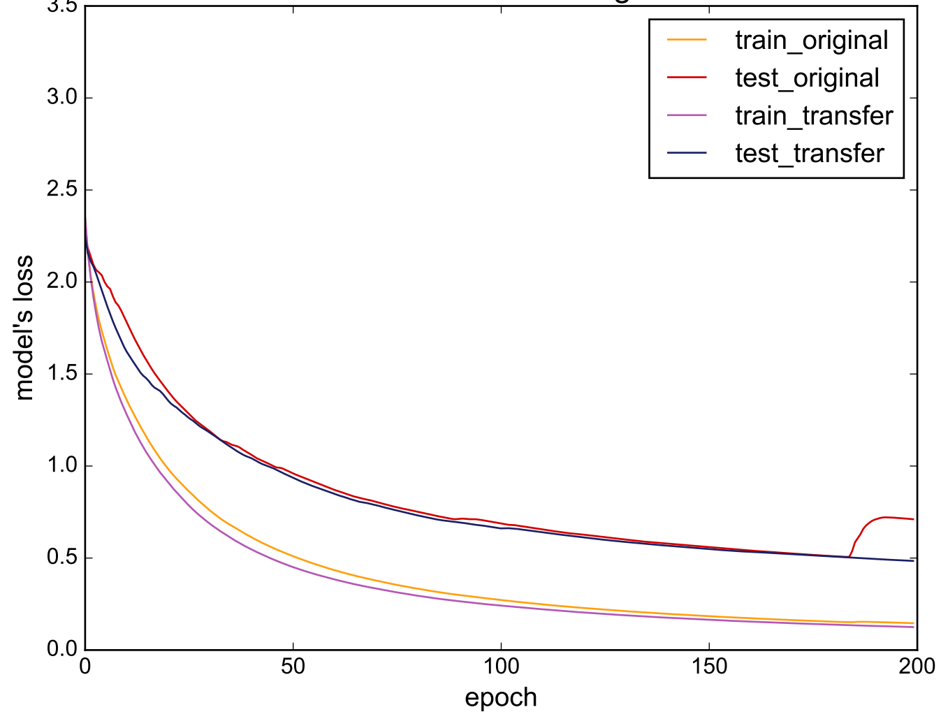
Source: DistalPhalanxTW - Target: FacesUCR
