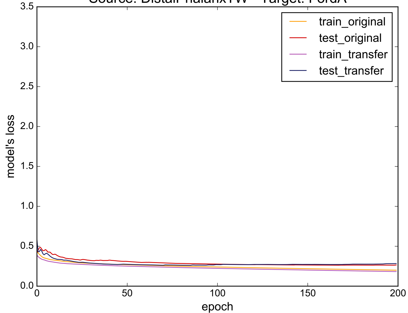
Source: DistalPhalanxTW - Target: FordA
