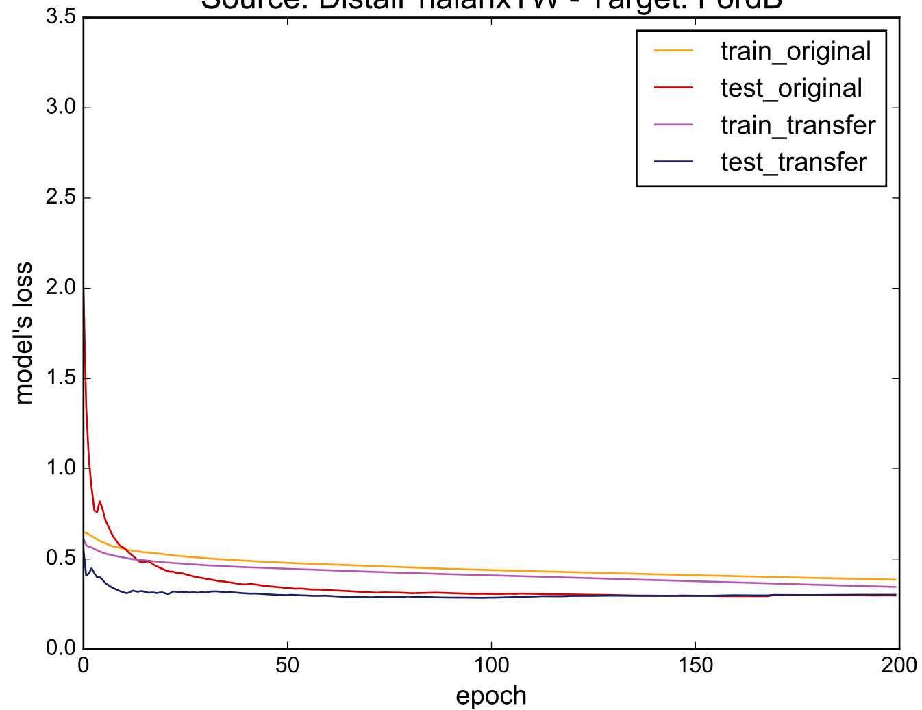
Source: DistalPhalanxTW - Target: FordB
