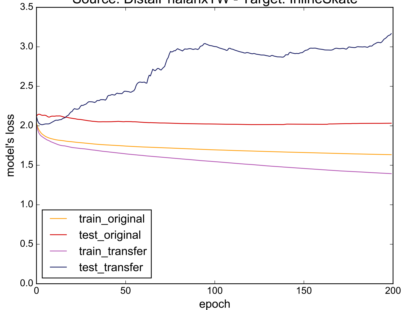
Source: DistalPhalanxTW - Target: InlineSkate
