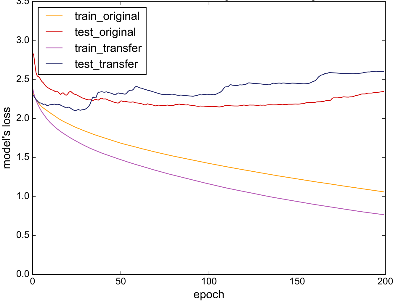
Source: DistalPhalanxTW - Target: InsectWingbeatSound
