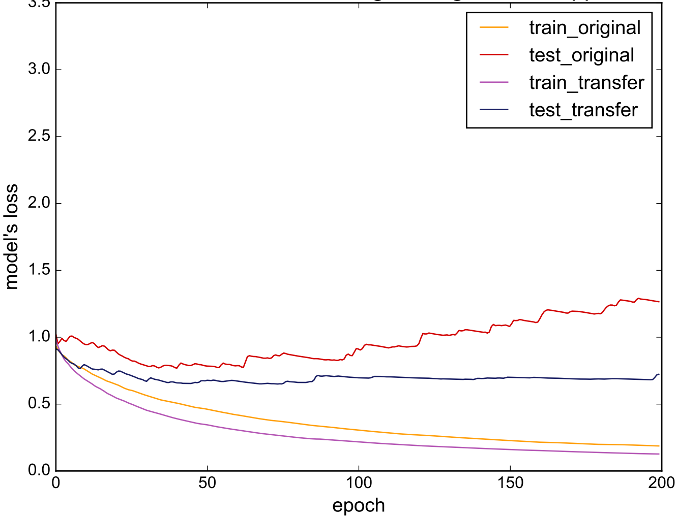
Source: DistalPhalanxTW - Target: LargeKitchenAppliances
