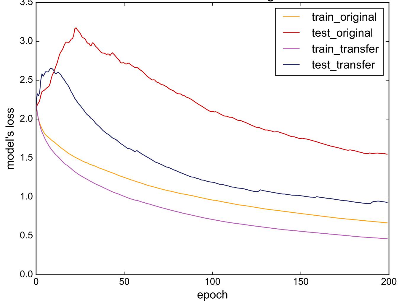
Source: DistalPhalanxTW - Target: MALLAT
