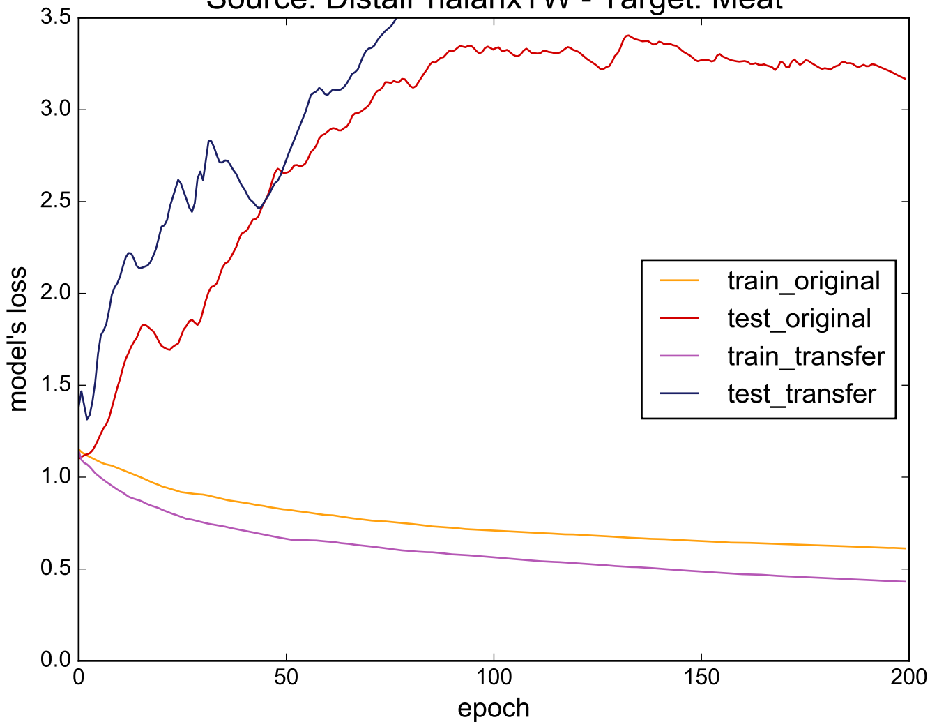
Source: DistalPhalanxTW - Target: Meat
