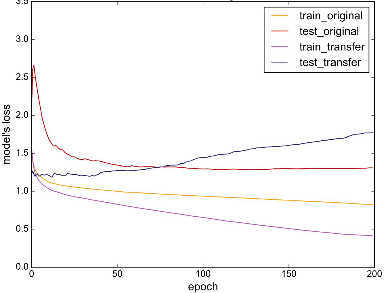
Source: DistalPhalanxTW - Target: MiddlePhalanxTW
