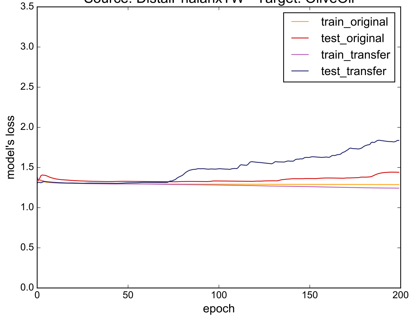
Source: DistalPhalanxTW - Target: OliveOil
