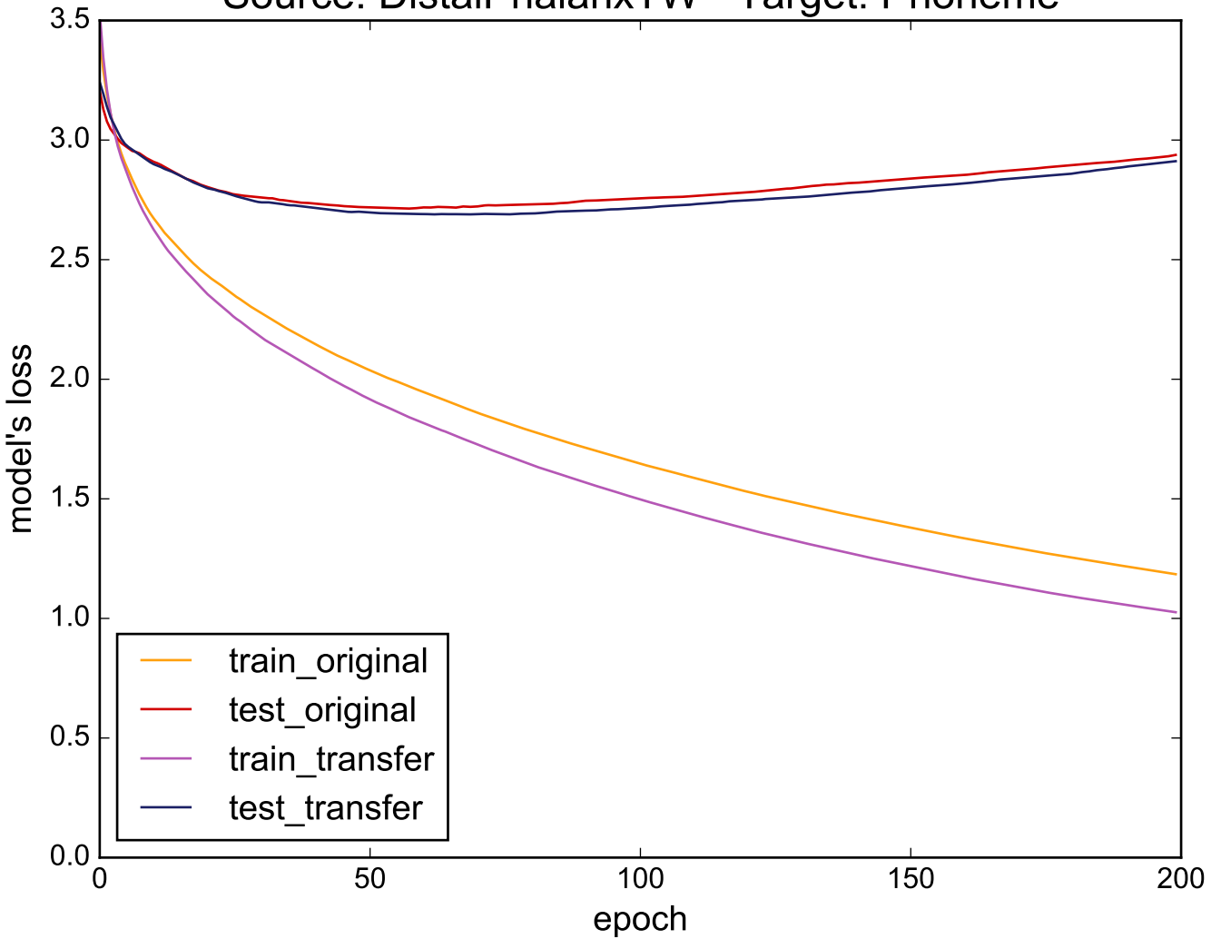
Source: DistalPhalanxTW - Target: Phoneme
