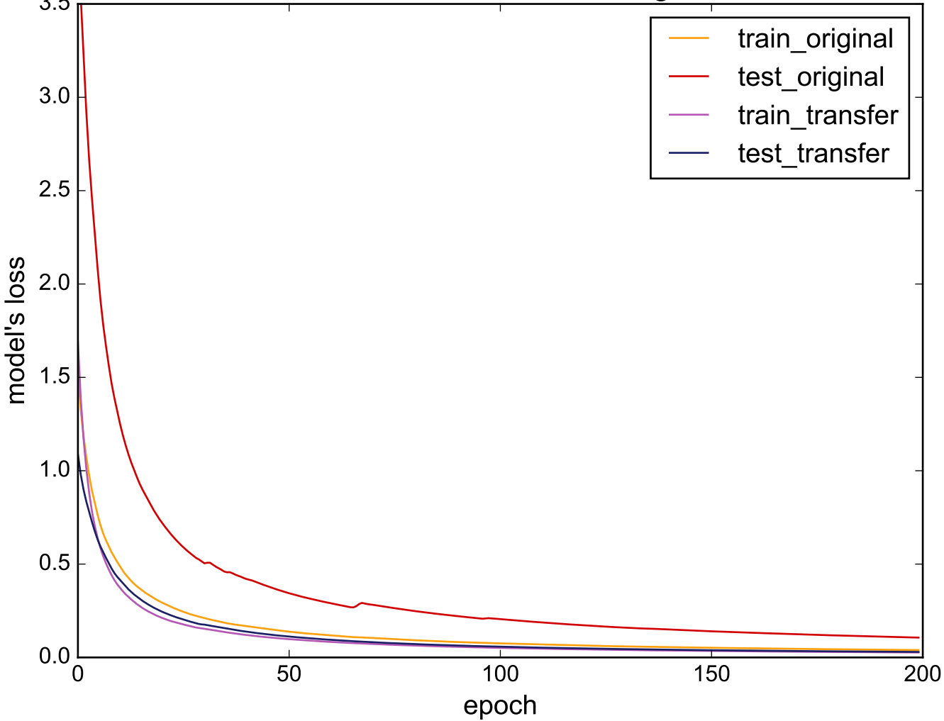
Source: DistalPhalanxTW - Target: Plane
