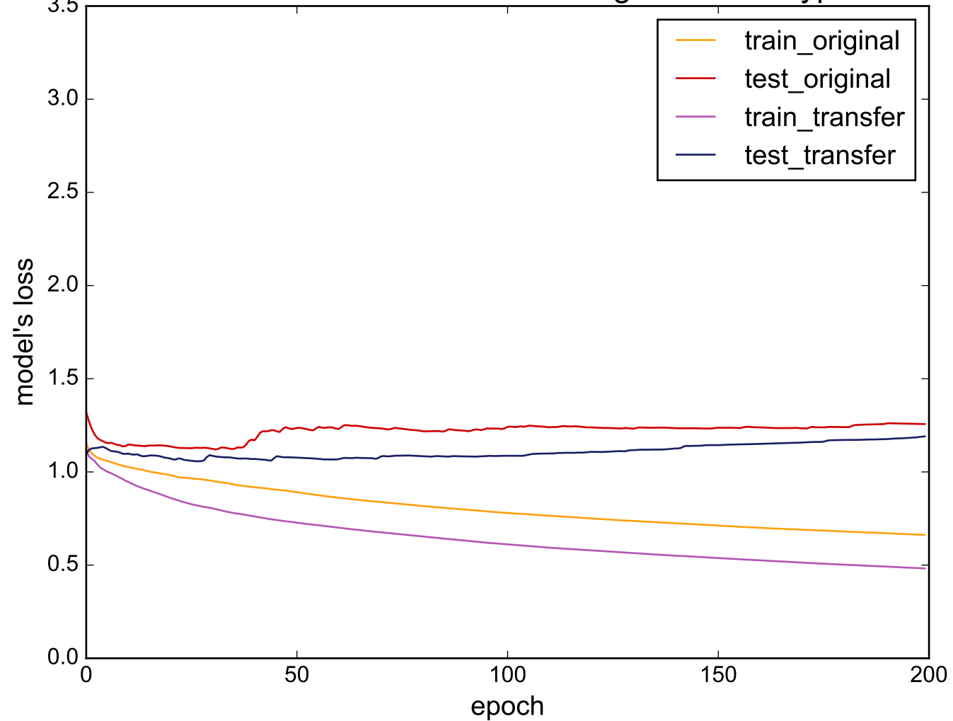
Source: DistalPhalanxTW - Target: ScreenType
