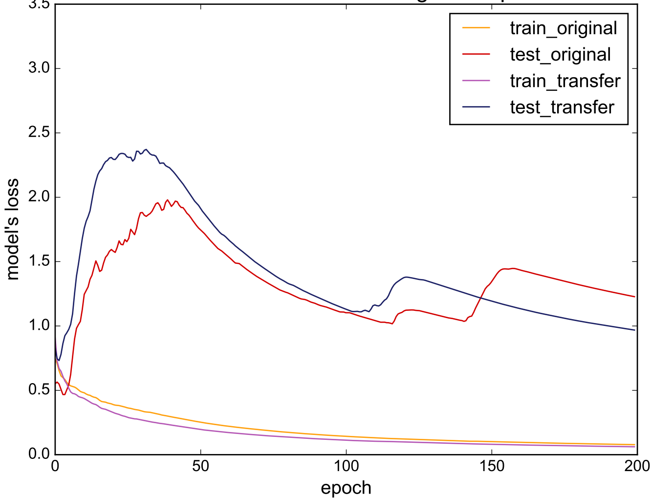
Source: DistalPhalanxTW - Target: ShapeletSim
