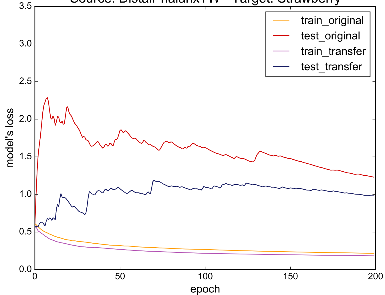
Source: DistalPhalanxTW - Target: Strawberry
