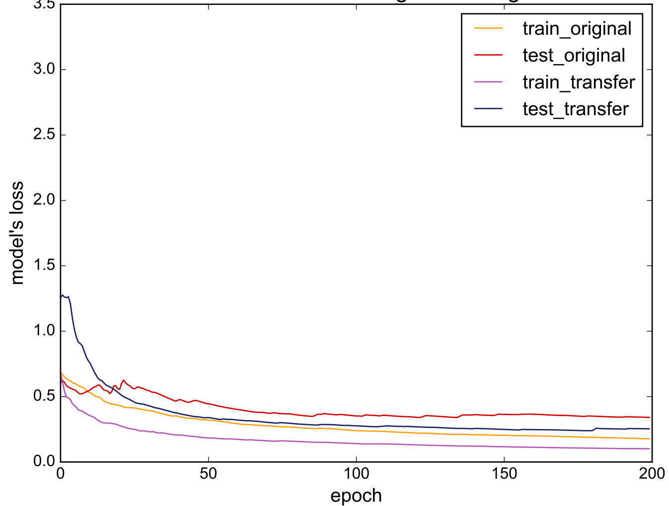
Source: DistalPhalanxTW - Target: ToeSegmentation1
