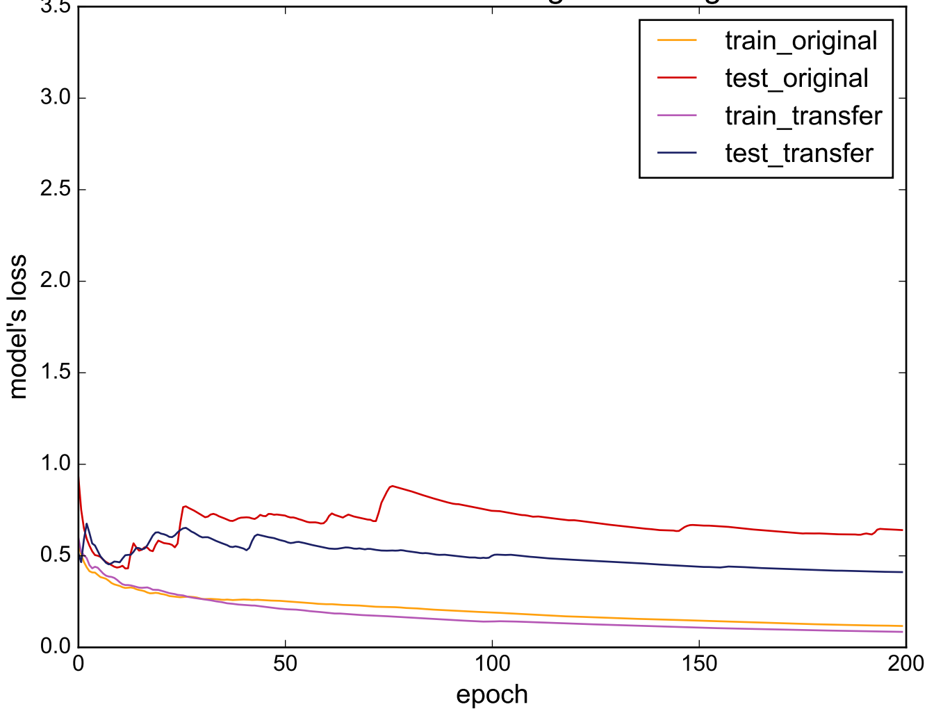
Source: DistalPhalanxTW - Target: ToeSegmentation2
