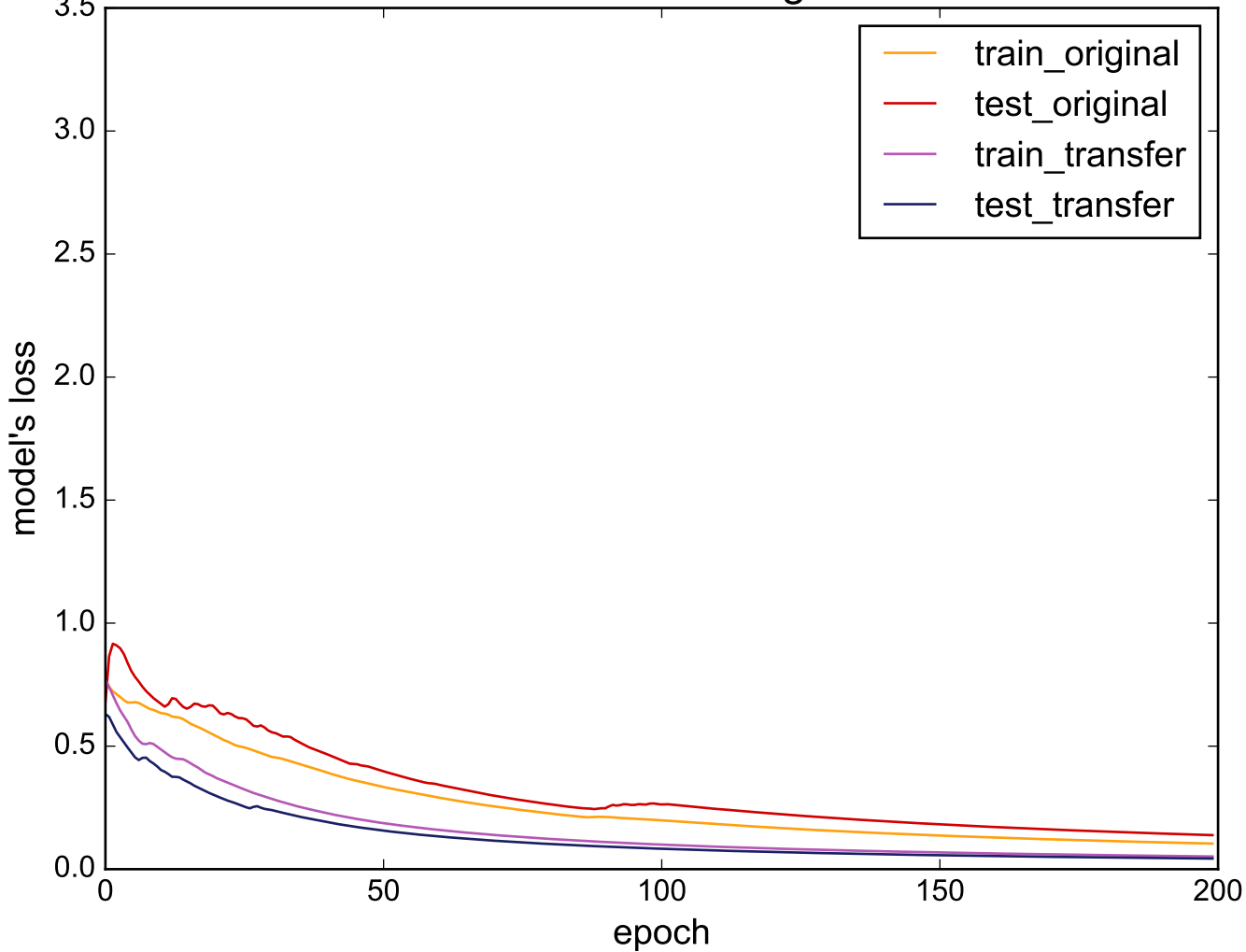
Source: DistalPhalanxTW - Target: TwoLeadECG
