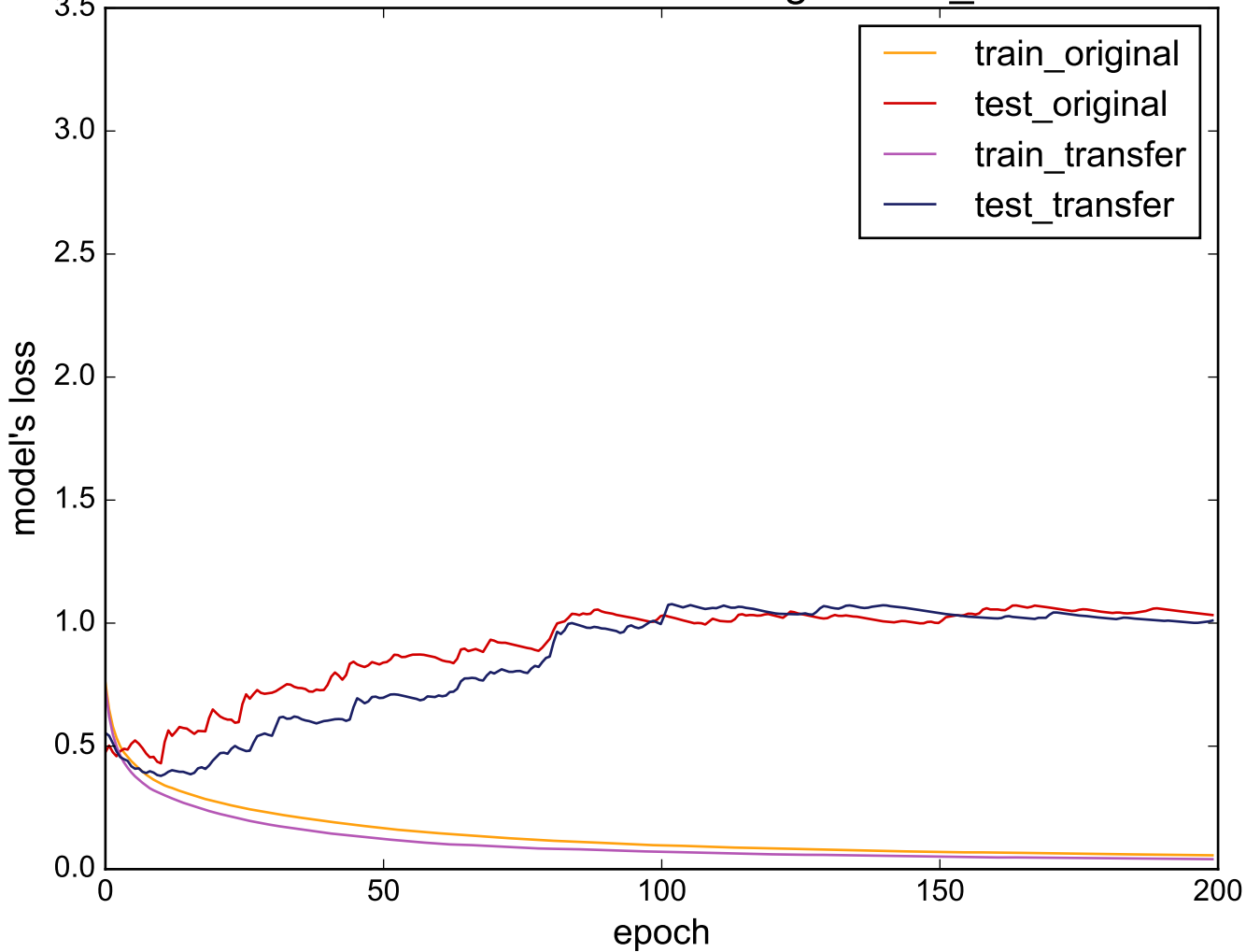
Source: DistalPhalanxTW - Target: Two_Patterns
