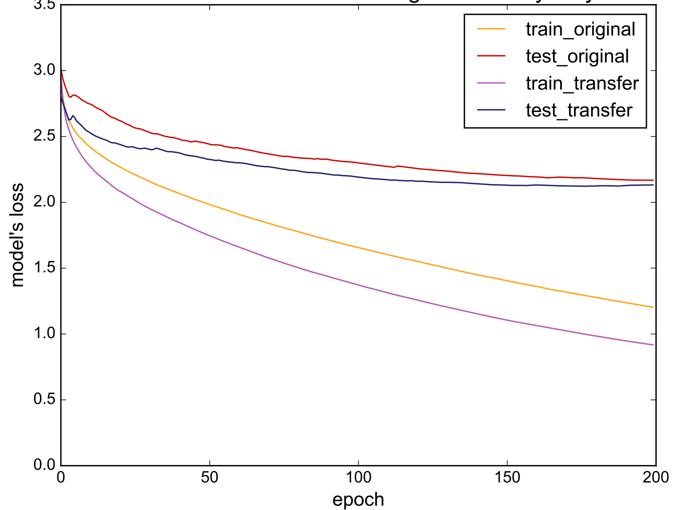
Source: DistalPhalanxTW - Target: WordsSynonyms
