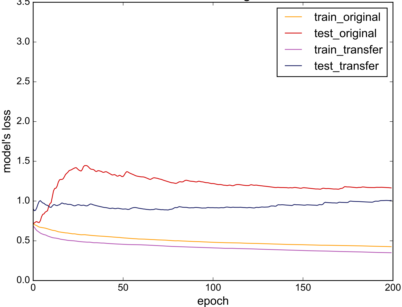
Source: DistalPhalanxTW - Target: WormsTwoClass
