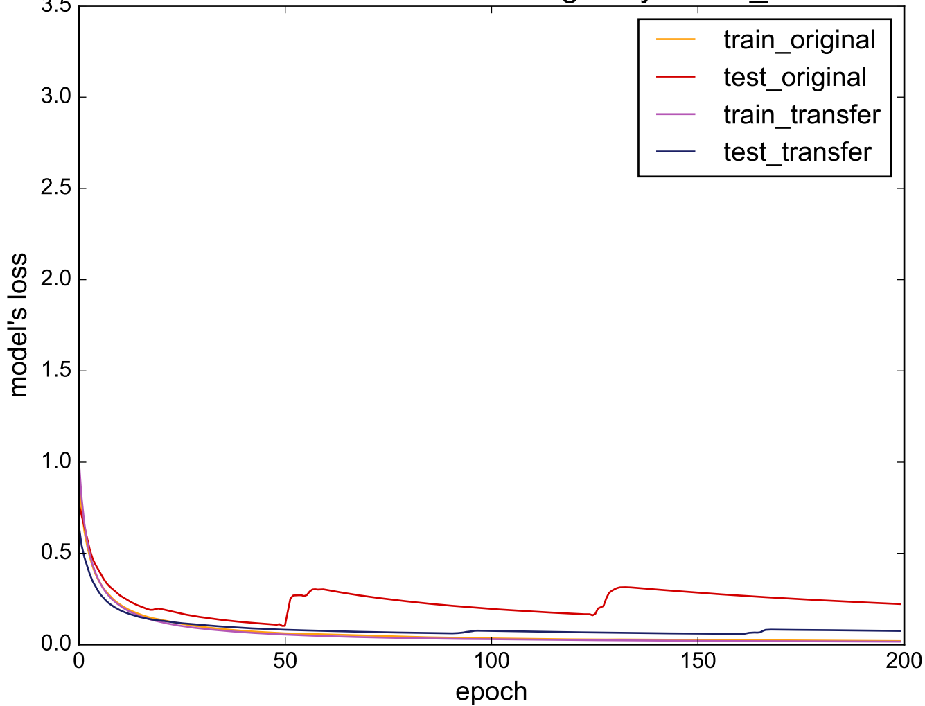
Source: DistalPhalanxTW - Target: synthetic_control
