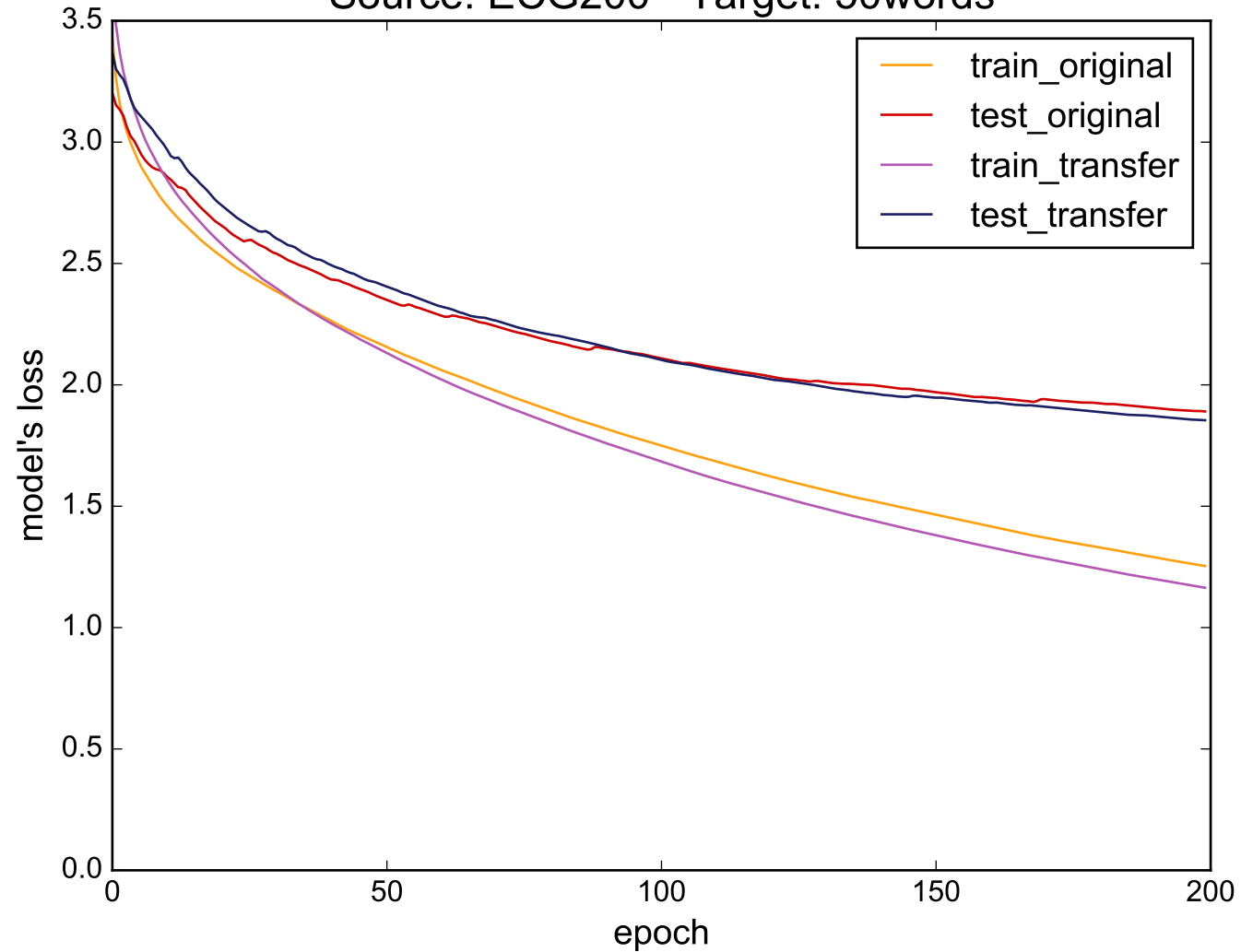
Source: ECG200 - Target: 50words
