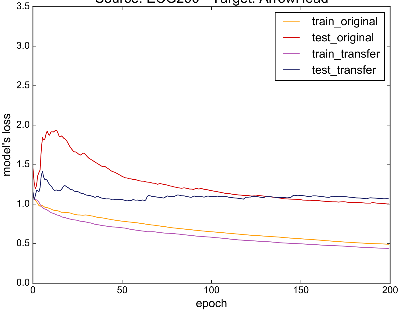
Source: ECG200 - Target: ArrowHead
