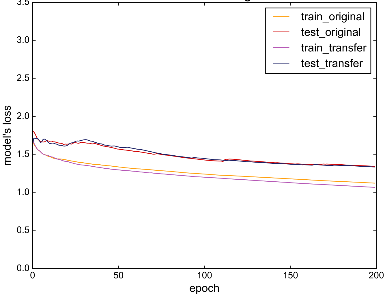
Source: ECG200 - Target: Beef
