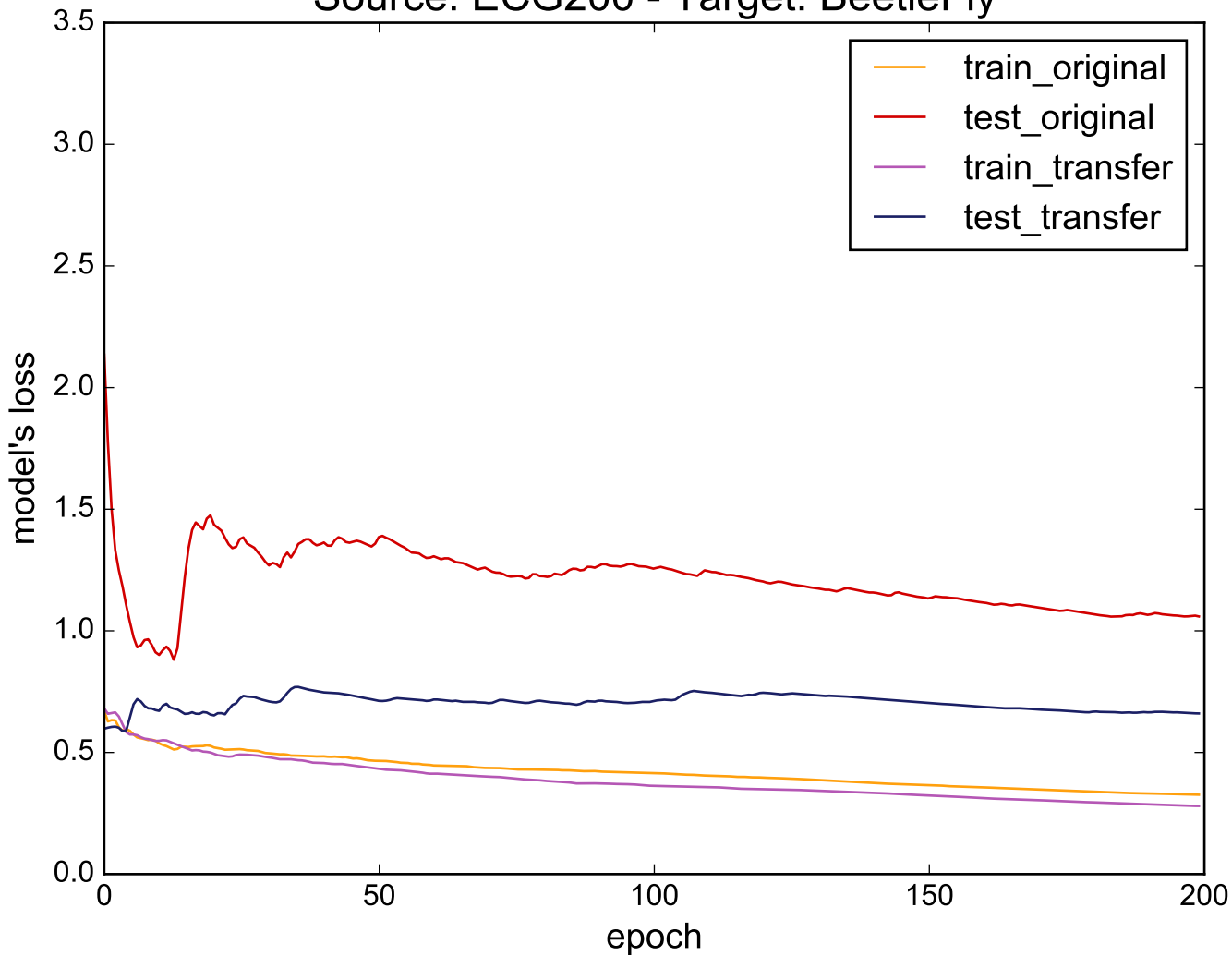
Source: ECG200 - Target: BeetleFly
