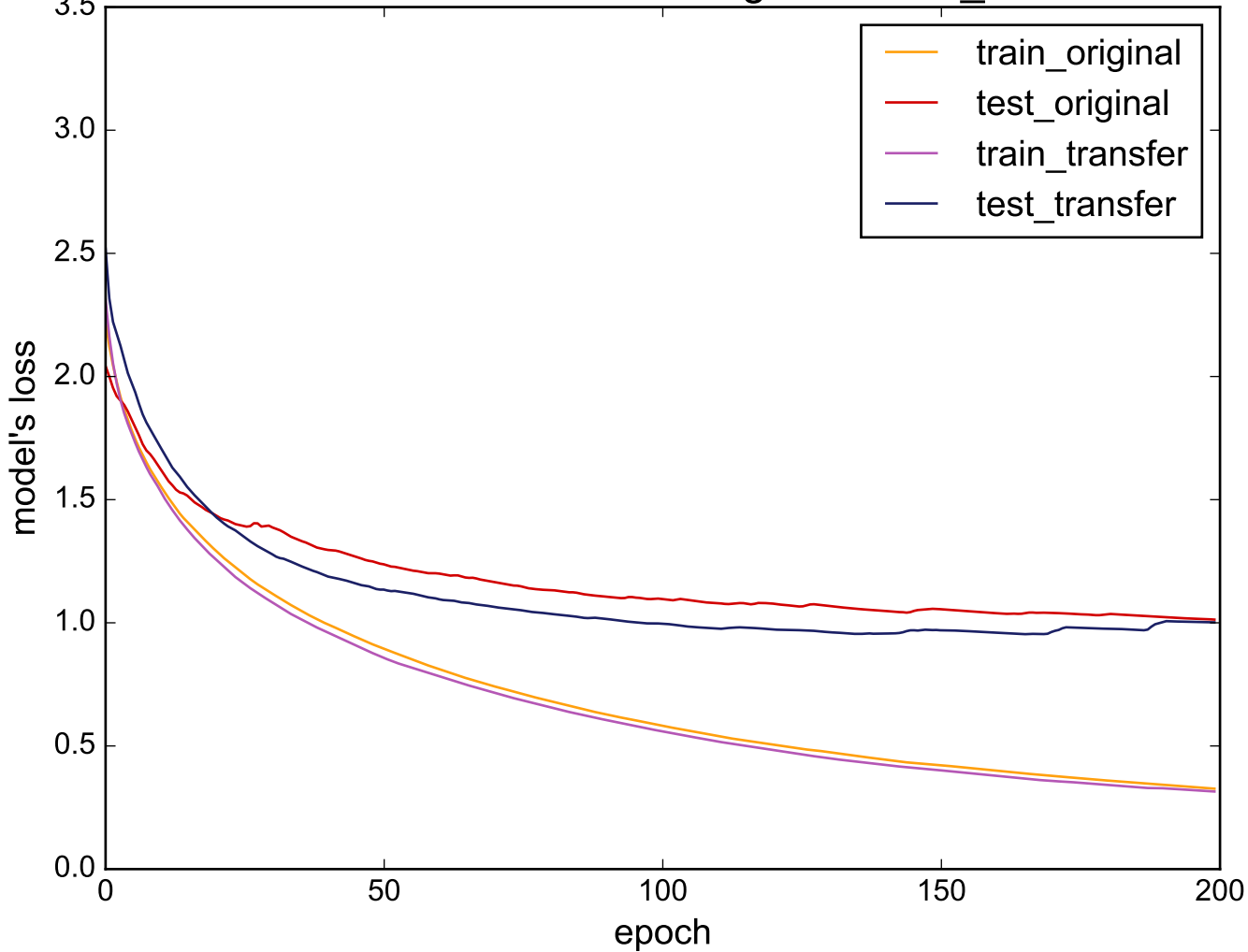
Source: ECG200 - Target: Cricket_X
