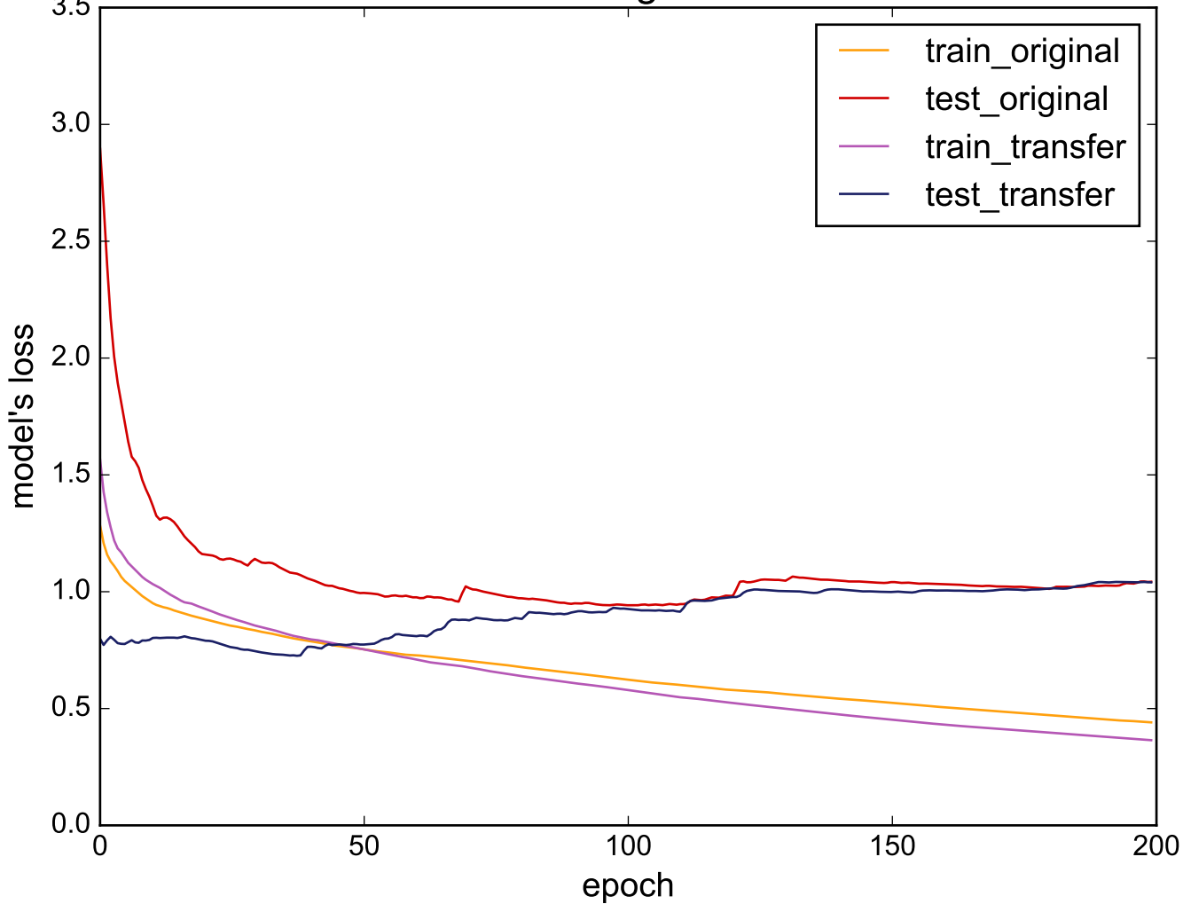
Source: ECG200 - Target: DistalPhalanxTW
