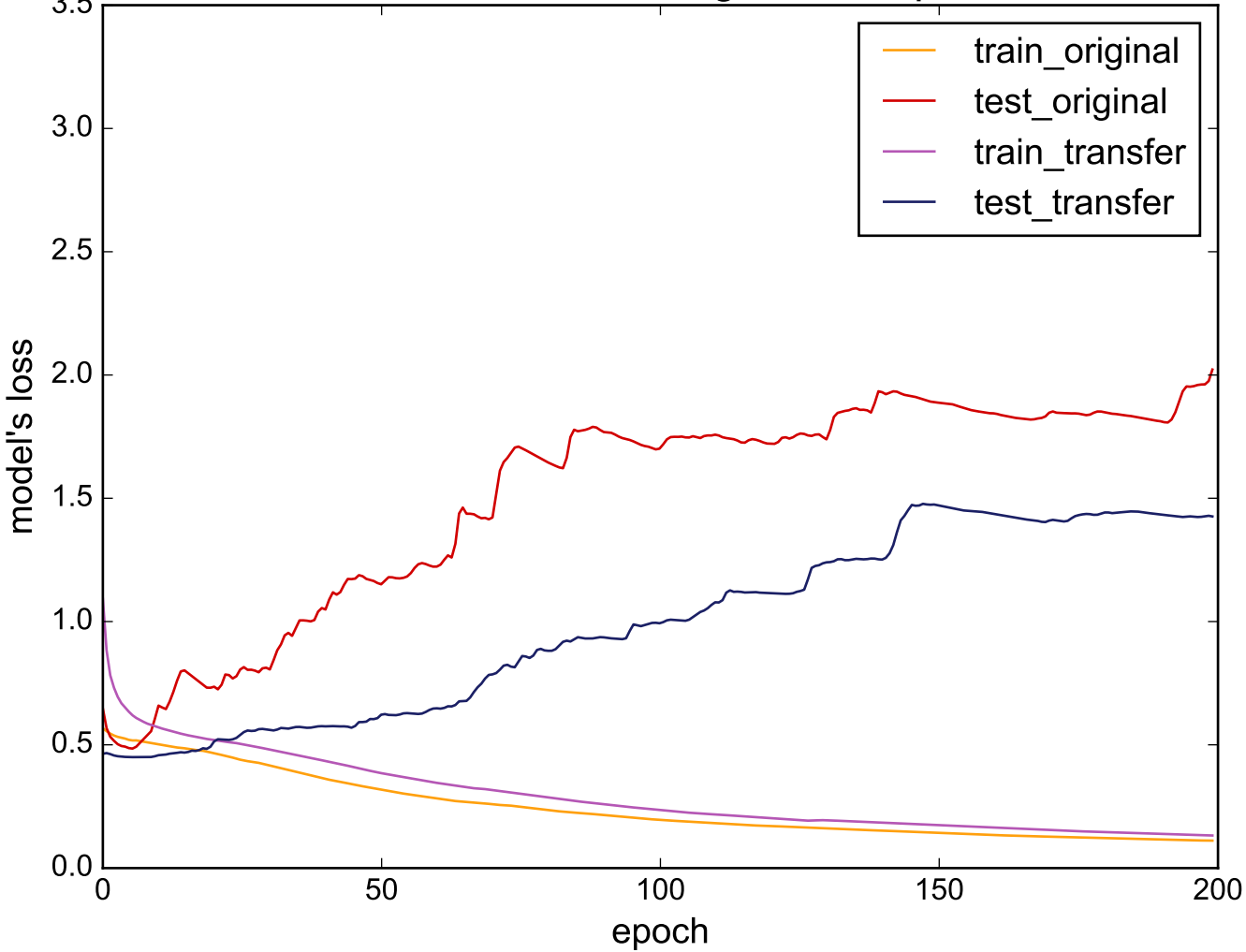
Source: ECG200 - Target: Earthquakes
