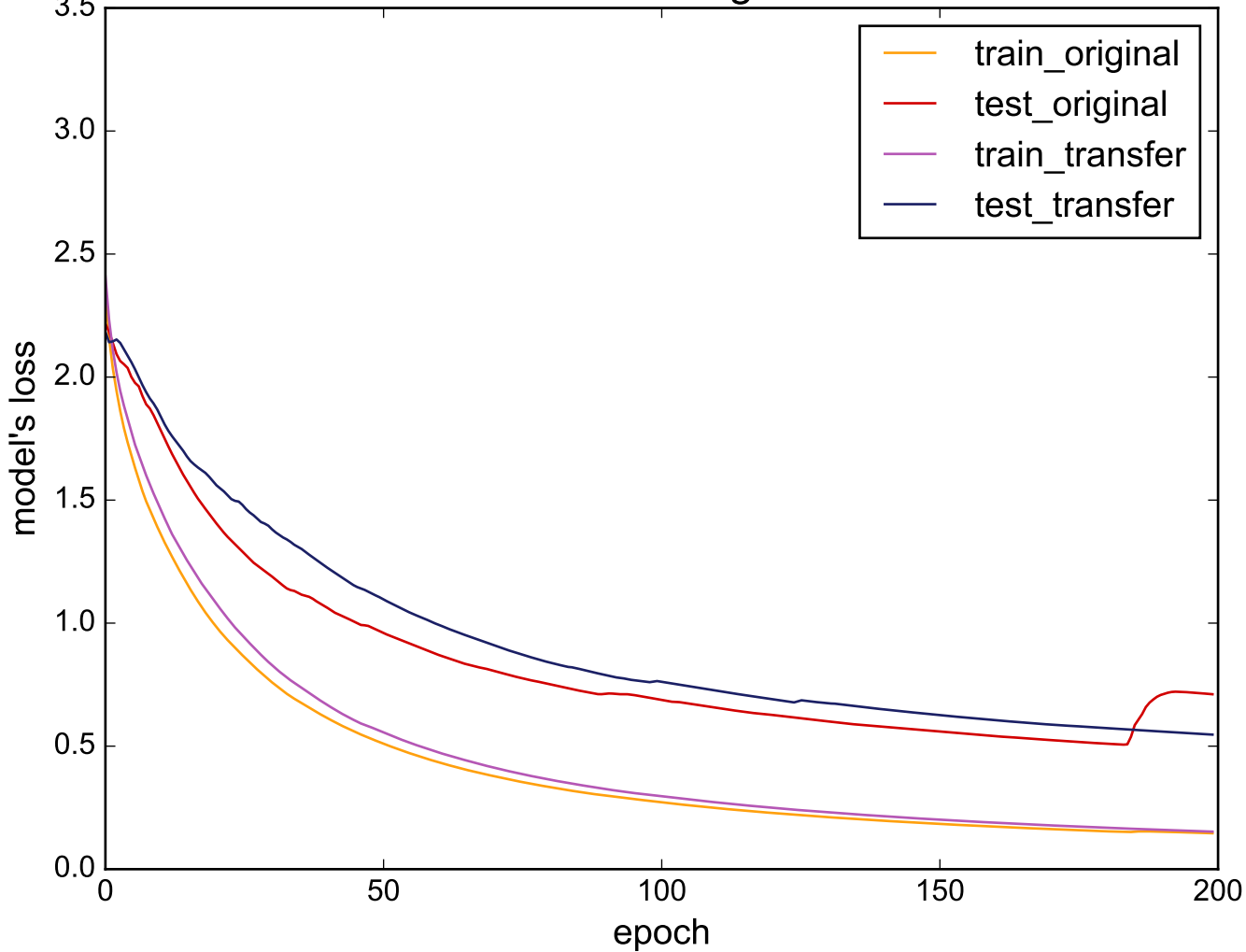
Source: ECG200 - Target: FacesUCR
