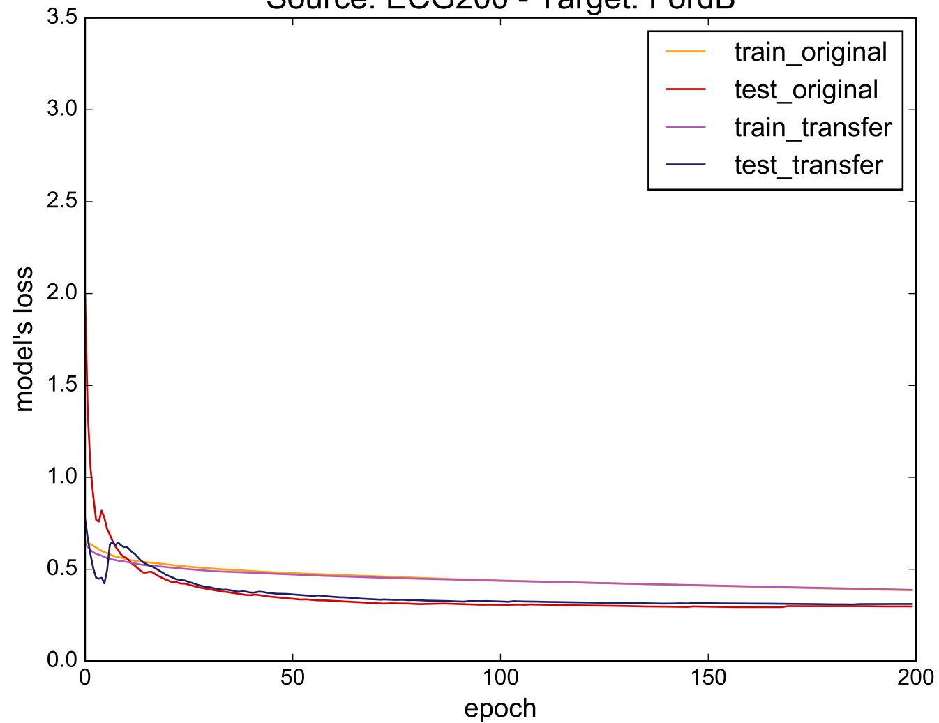
Source: ECG200 - Target: FordB
