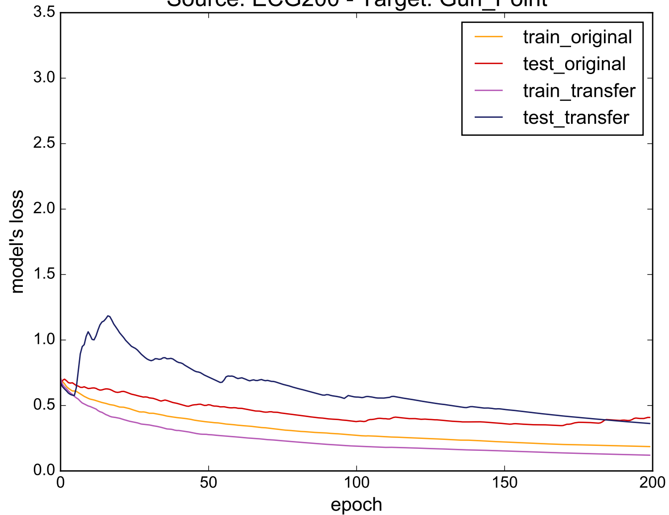
Source: ECG200 - Target: Gun_Point
