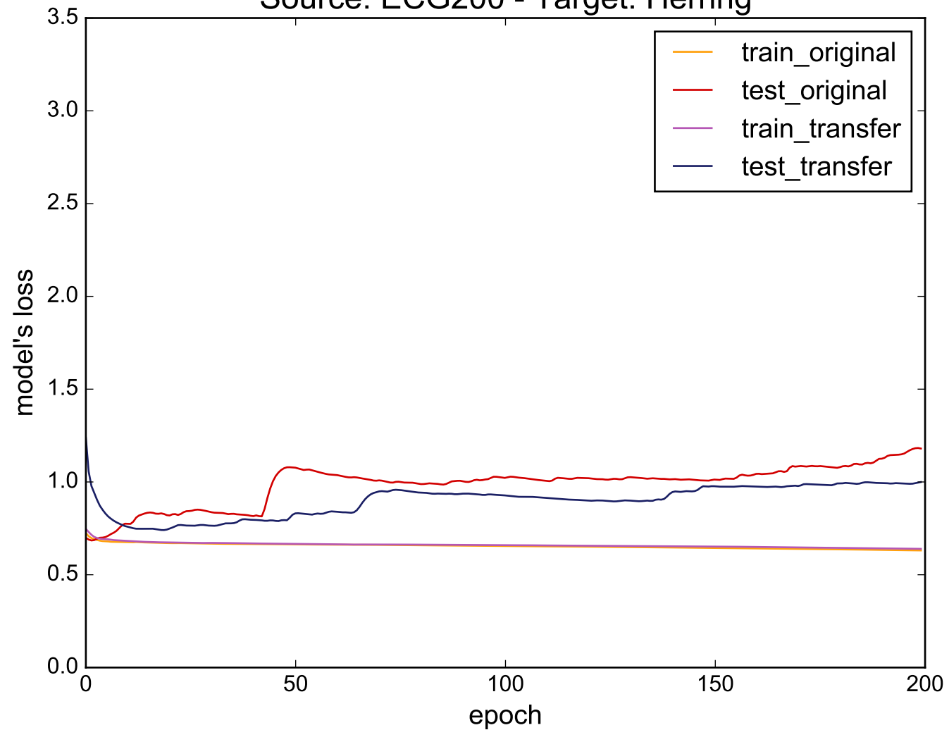
Source: ECG200 - Target: Herring
