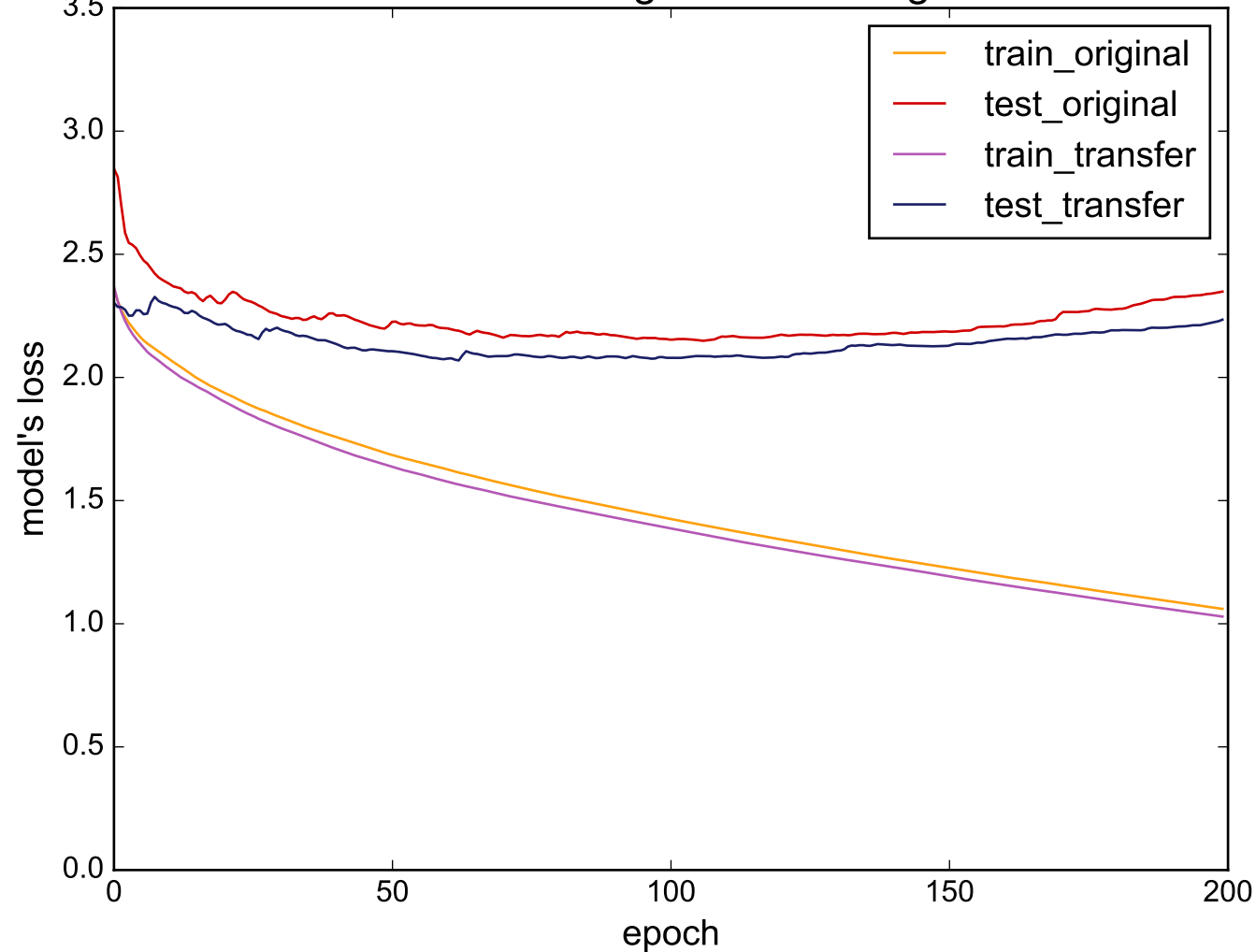
Source: ECG200 - Target: InsectWingbeatSound
