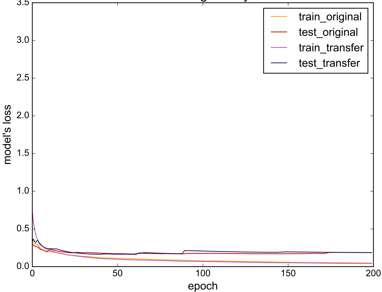
Source: ECG200 - Target: ItalyPowerDemand
