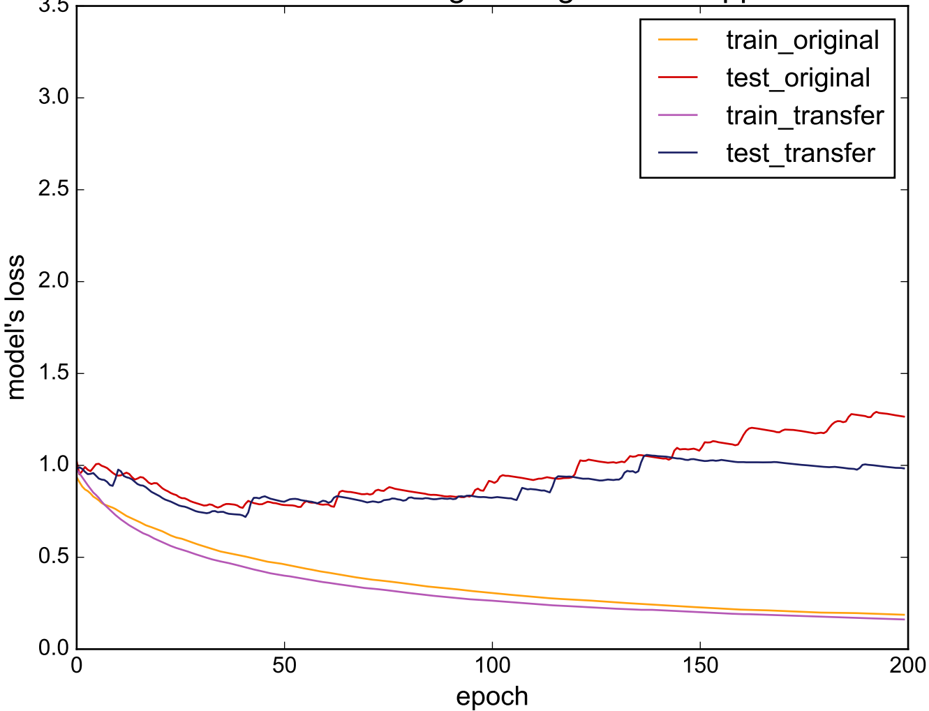
Source: ECG200 - Target: LargeKitchenAppliances
