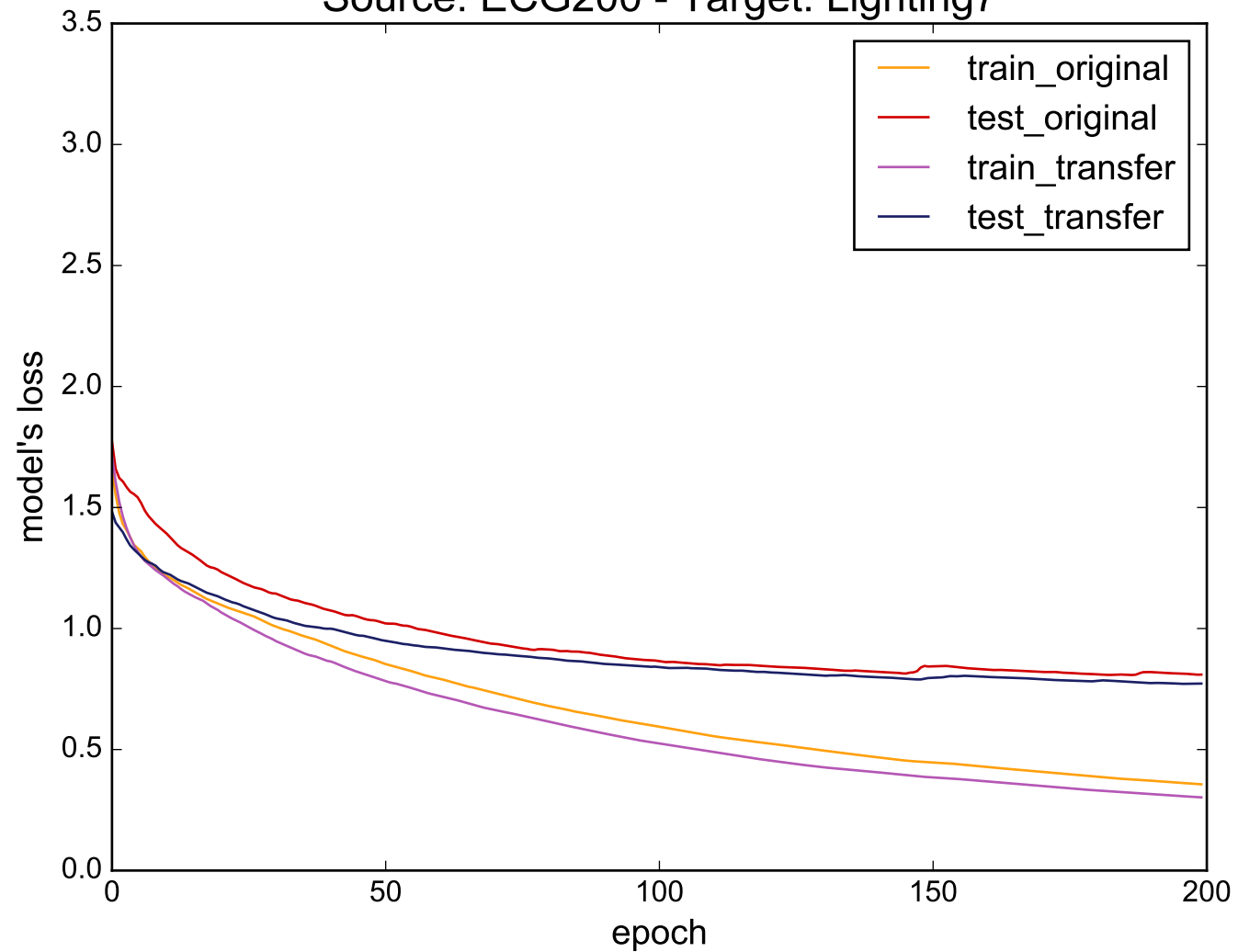
Source: ECG200 - Target: Lighting7
