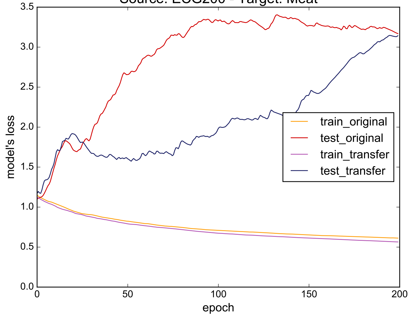
Source: ECG200 - Target: Meat
