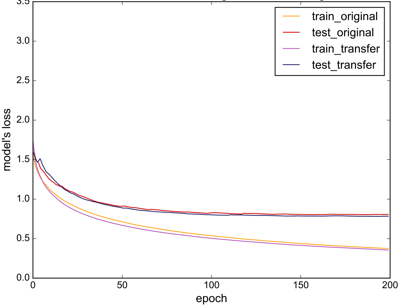
Source: ECG200 - Target: MedicalImages
