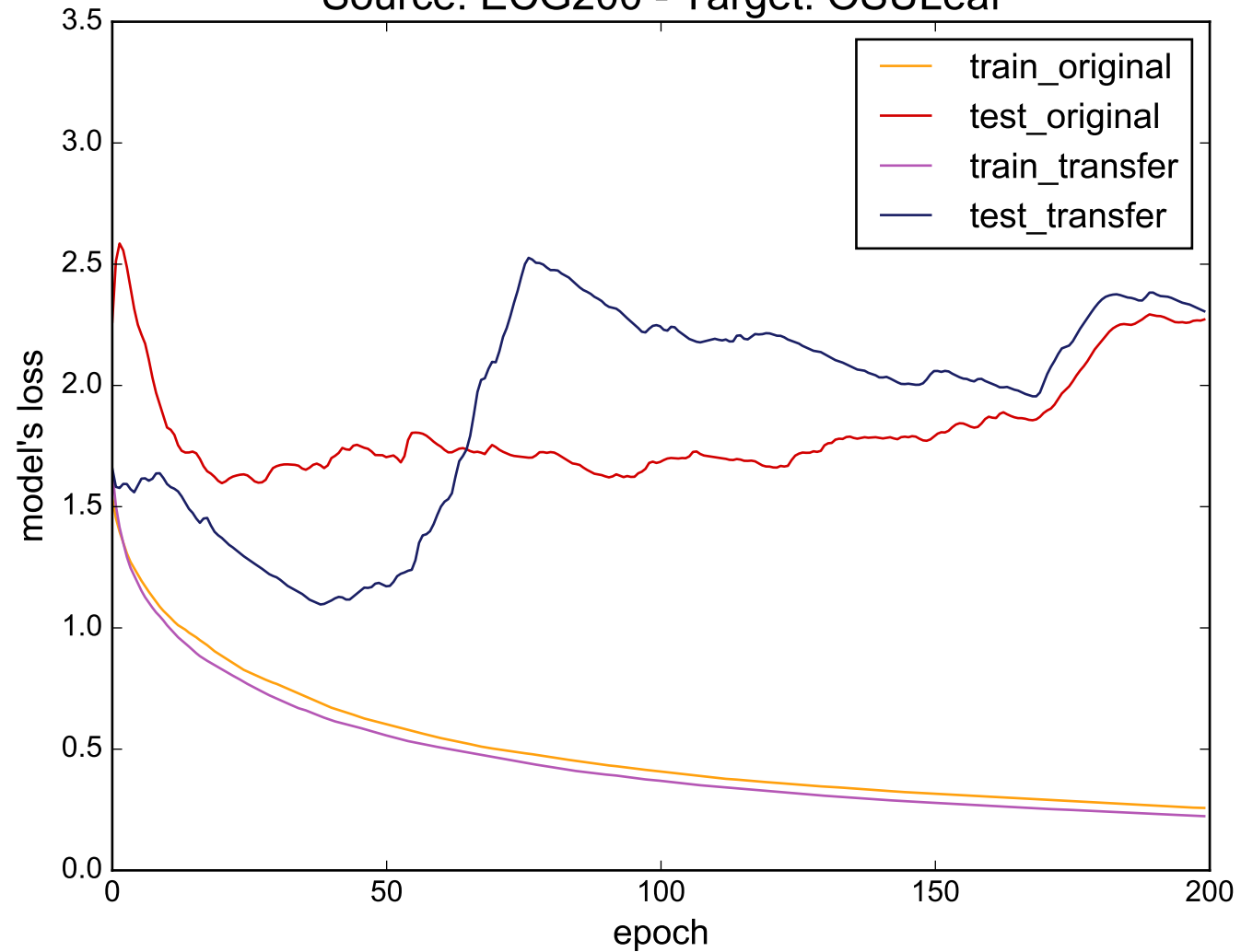
Source: ECG200 - Target: OSULeaf
