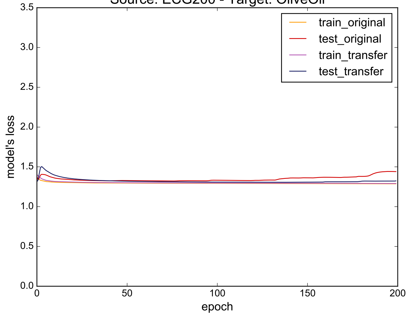
Source: ECG200 - Target: OliveOil
