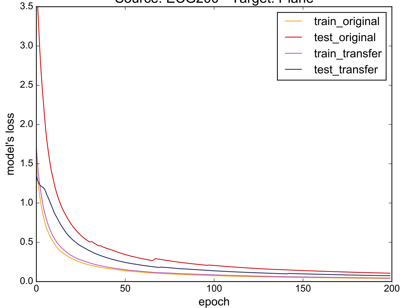
Source: ECG200 - Target: Plane
