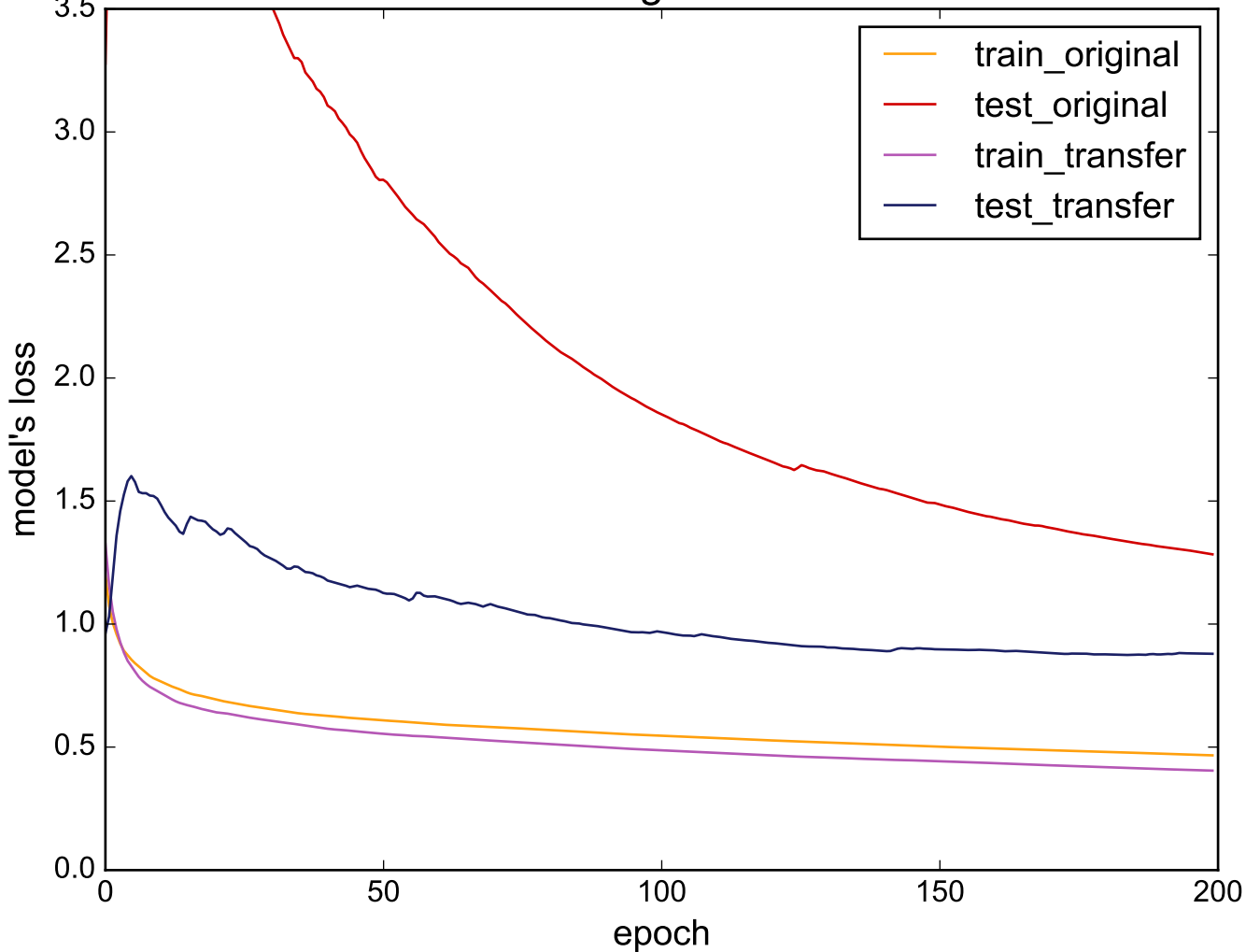
Source: ECG200 - Target: ProximalPhalanxTW
