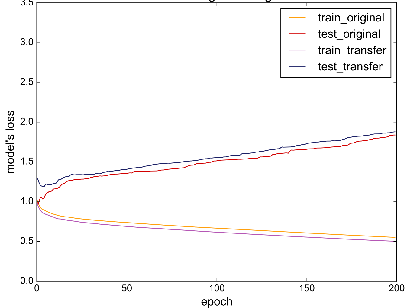
Source: ECG200 - Target: RefrigerationDevices
