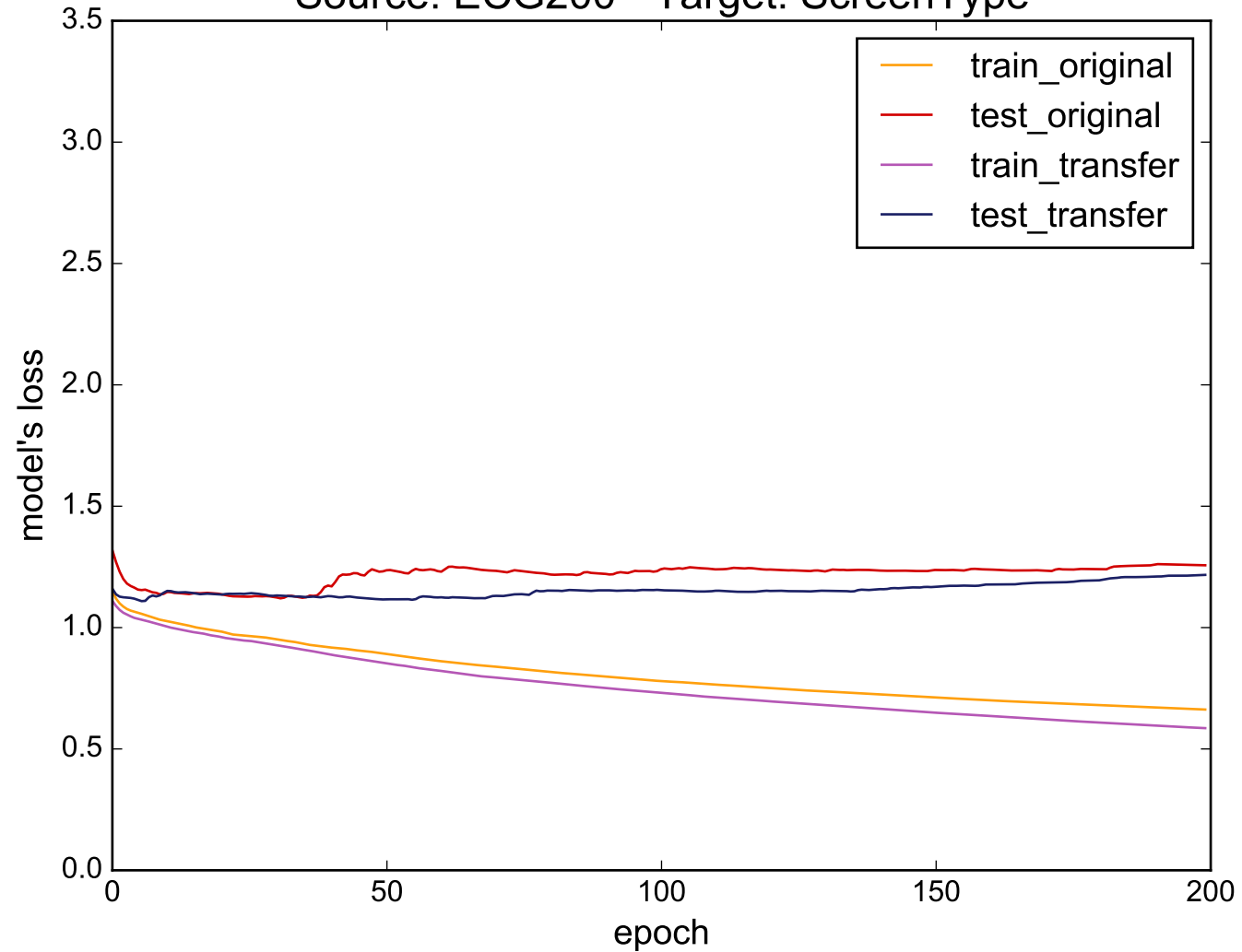
Source: ECG200 - Target: ScreenType
