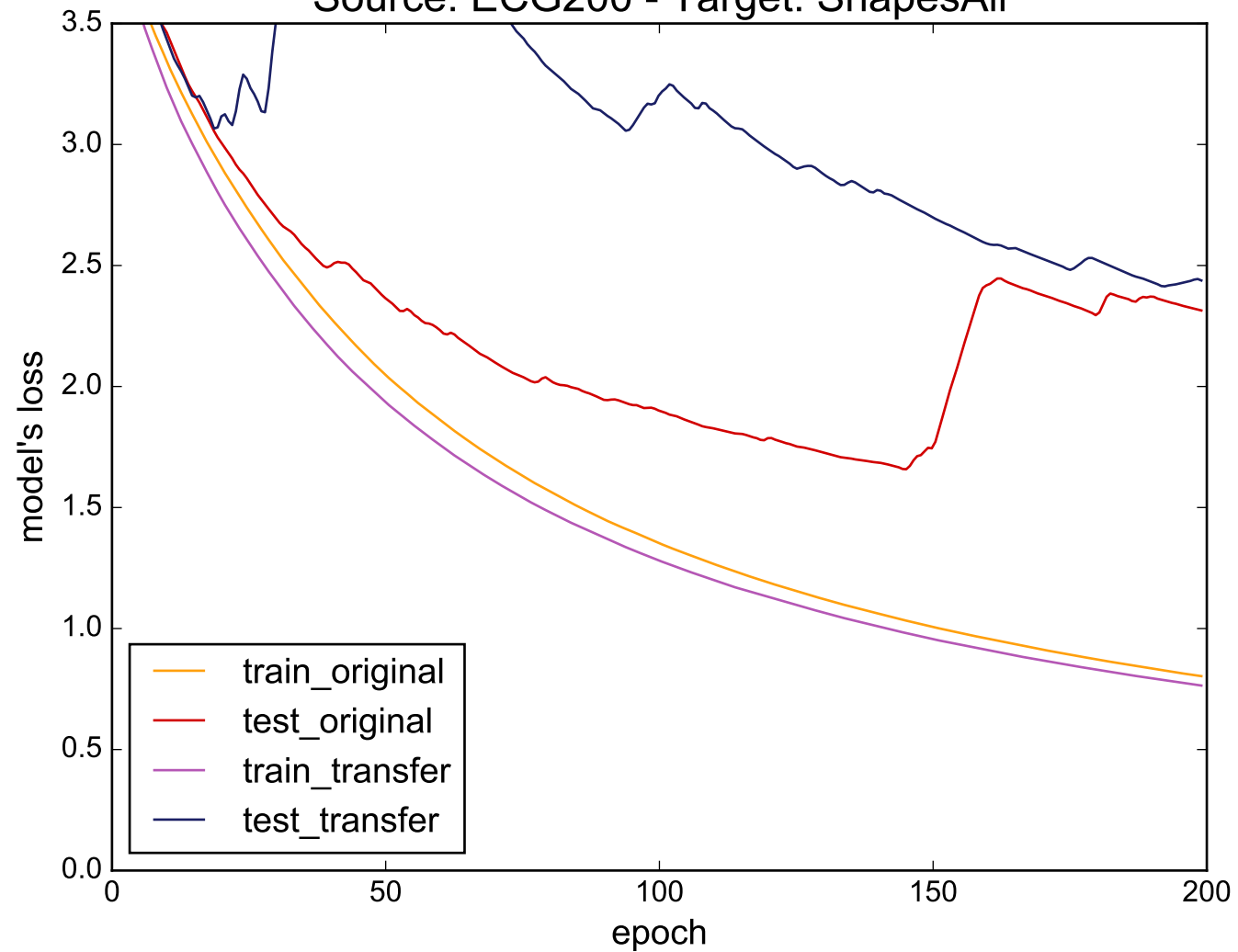
Source: ECG200 - Target: ShapesAll
