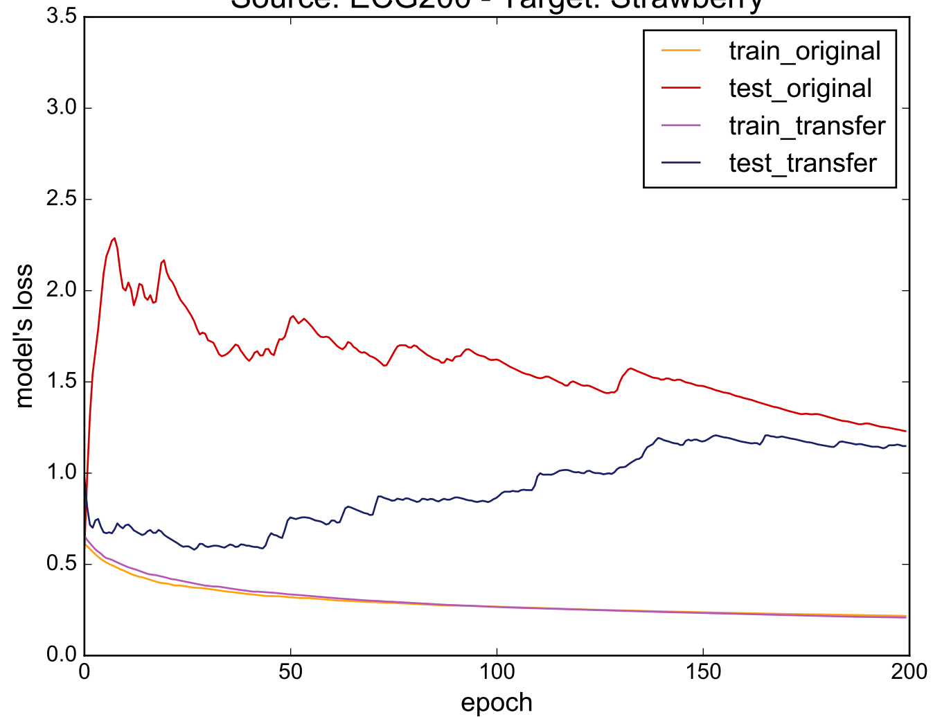
Source: ECG200 - Target: Strawberry
