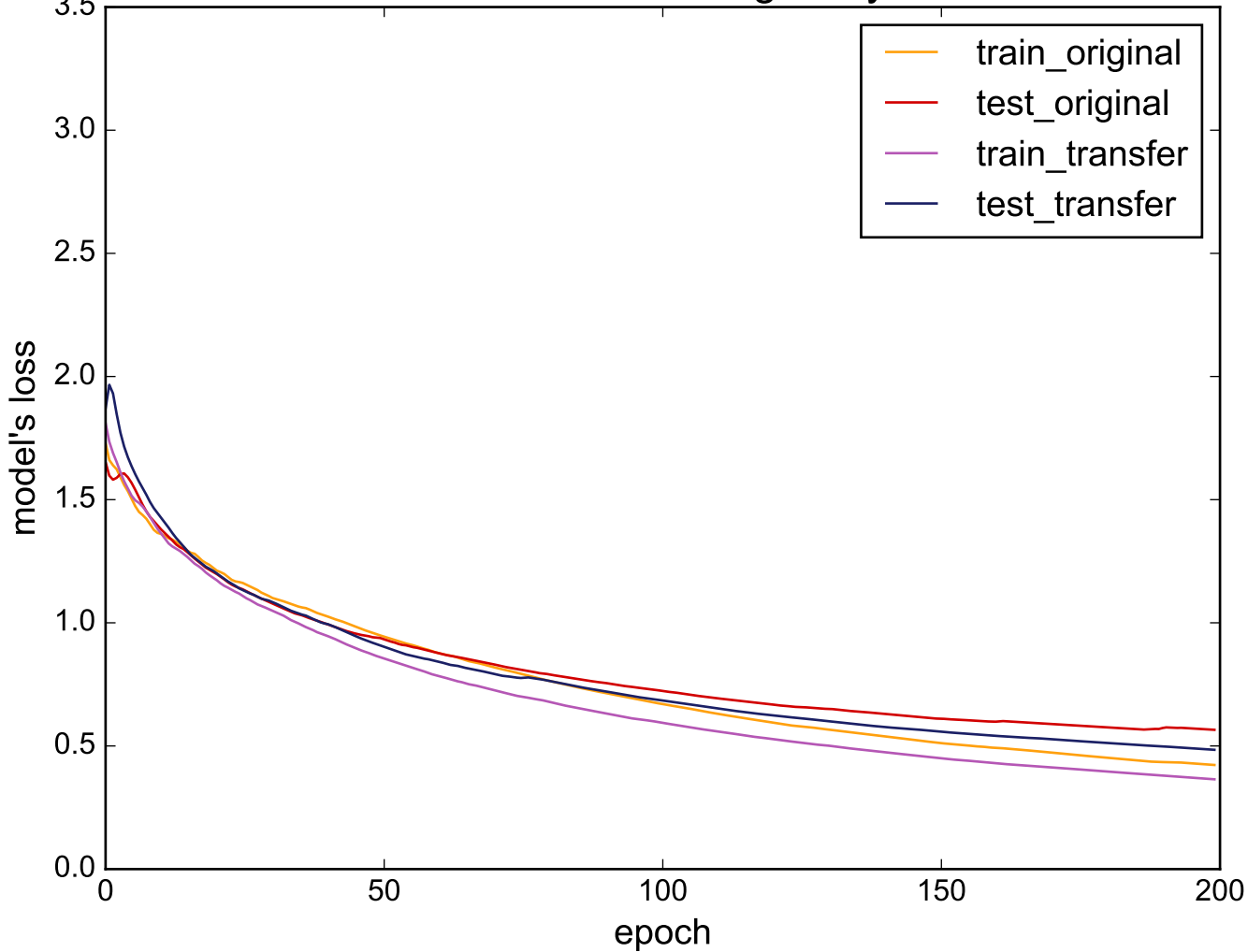
Source: ECG200 - Target: Symbols
